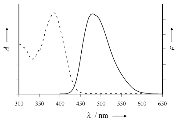
Figure 1. Normalized absorption (---) ( 2.5 \times 10^{-5} \text{ M} ) and fluorescence (—) ( 2.5 \times 10^{-6} \text{ M} , \lambda_{\text{ex}} = 386 \text{ nm} ) spectra of 2 in benzene. Measured under oxygen-free conditions.
