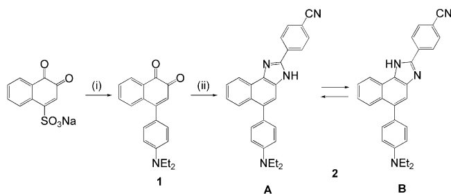
Scheme 1. (i) N,N -diethylaniline, \text{NiCl}_2 \cdot 4\text{H}_2\text{O} , \text{CH}_3\text{COOH}/\text{H}_2\text{O} (4:1), 7 d, room temp., 58%; (ii) p -cyanobenzaldehyde, \text{CH}_3\text{COONH}_4 , \text{CH}_3\text{COOH} , 1 h, 80 °C, 75%.
