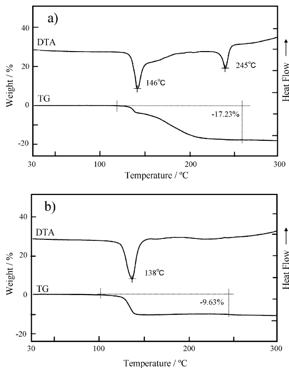
Figure 2. TG and DTA traces for the guest inclusion compounds: (a) 2 -morpholine and (b) 2 -ethanol.
