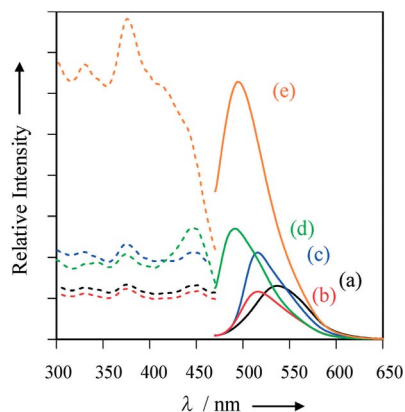
Figure 3. Solid-state excitation (---) and fluorescence (—) spectra of the guest-free and guest inclusion crystals of 2 : (a) 2 (guest-free): \lambda_{\text{ex}} = 451 nm, \lambda_{\text{em}} = 536 nm, \Phi = 0.06 ; (b) 2 -morpholine: \lambda_{\text{ex}} = 452 nm, \lambda_{\text{em}} = 517 nm, \Phi = 0.05 ; (c) 2 -ethanol: \lambda_{\text{ex}} = 451 nm, \lambda_{\text{em}} = 515 nm, \Phi = 0.08 ; (d) 2 -ethyl acetate: \lambda_{\text{ex}} = 446 nm, \lambda_{\text{em}} = 491 nm, \Phi = 0.10 ; (e) 2 -1,4-dioxane: \lambda_{\text{ex}} = 440 nm, \lambda_{\text{em}} = 495 nm, \Phi = 0.26 .
