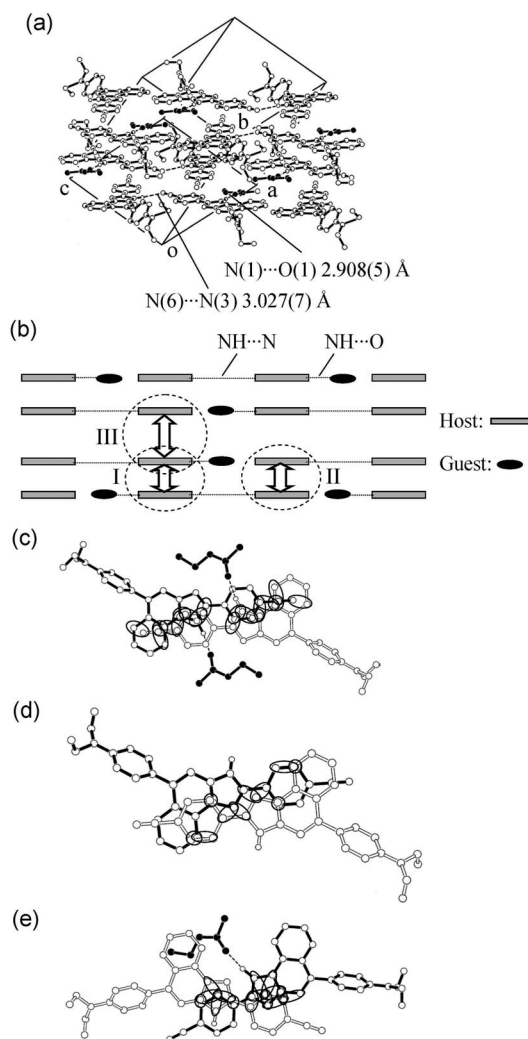
Figure 7. Crystal structure of 2 -ethyl acetate: (a) a stereoview of the molecular packing structure; (b) schematic structure; (c) top view of the pairs of fluorophores with form B (stacking I); (d) with form A (stacking II); (e) \pi stacking between the host with form A and the host with form B (stacking III).
