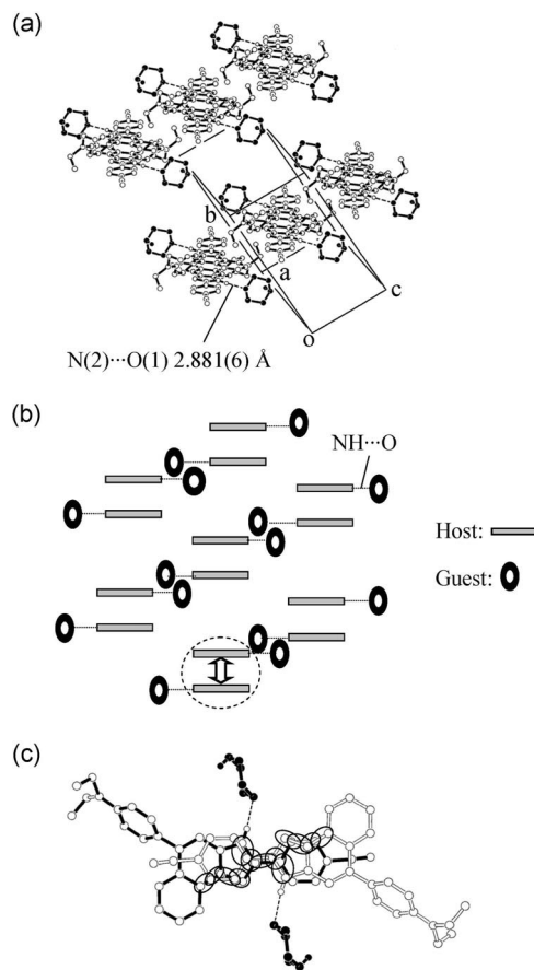
Figure 5. Crystal structure of 2 ·morpholine: (a) a stereoview of the molecular packing structure; (b) schematic structure; (c) top view of the pairs of fluorophores.
