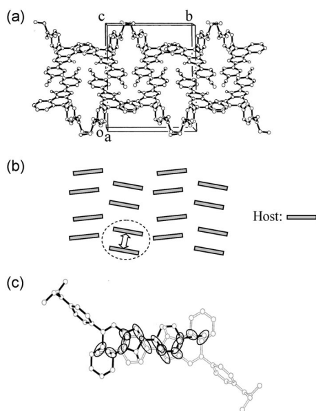
Figure 4. Crystal structure of 2 : (a) a stereoview of the molecular packing structure; (b) schematic structure; (c) top view of the pairs of fluorophores.
