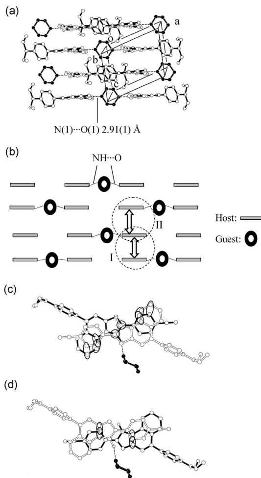
Figure 8. Crystal structure of 2 ·1,4-dioxane: (a) a stereoview of the molecular packing structure; (b) schematic structure; (c) (stacking I) and (d) (stacking II) top view of the \pi stacking between the fluorophores.
