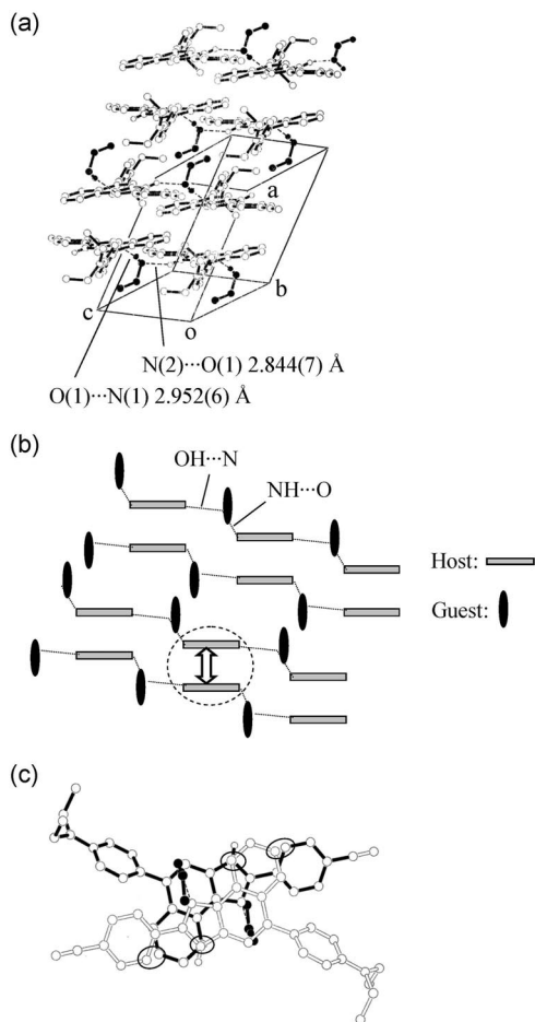
Figure 6. Crystal structure of 2 -ethanol: (a) a stereoview of the molecular packing structure; (b) schematic structure; (c) top view of the pairs of fluorophores.
